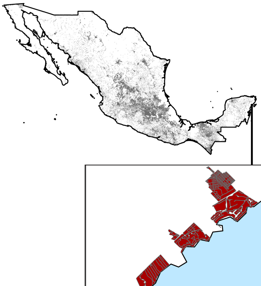
ADM 6/0 boundaries for all of Mexico; Inset: detail over Tulum (area in red included in sample)
